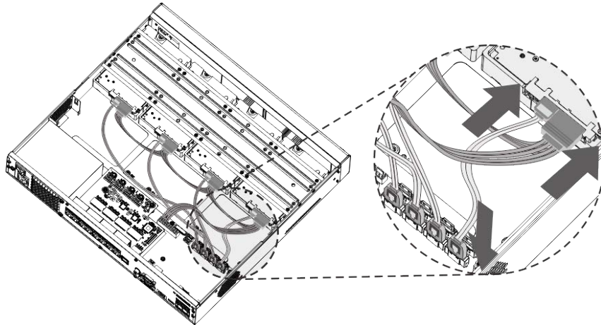
Figure 2-22 Connect cables
