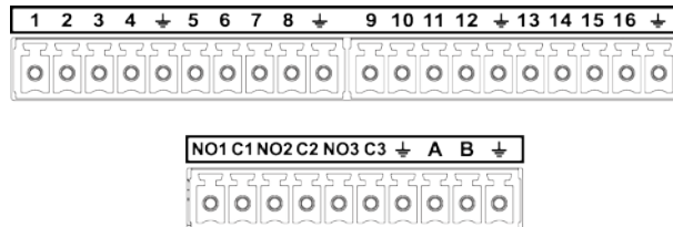
Figure 4-2 Alarm ports
