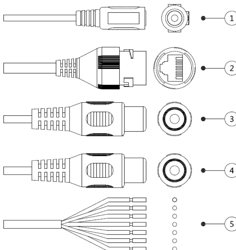
Figure 1-1 Cable list
