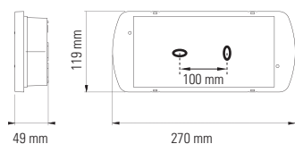
UNILED 2-45 et 2-400 (mm)
