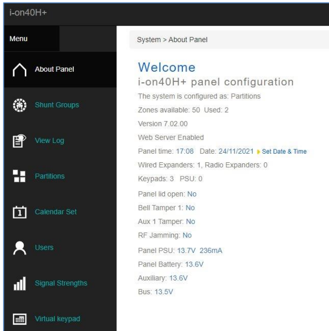
Figure 1 - Interface Web
